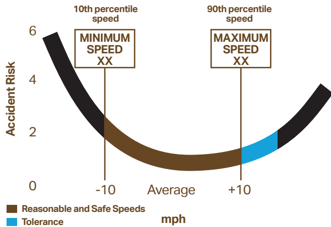
Figure 4: Speed limit setting 93
