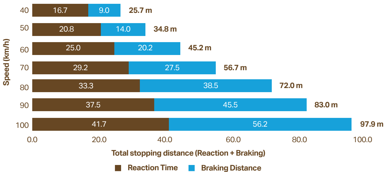
Figure 2: Total stopping distance in ideal weather conditions on dry asphalt 79
