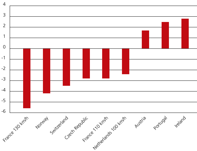
Fig. 18 Percentage changes in the mean speeds on motorways. Source: National data (see Table 11, Table 14 in the Annex)
